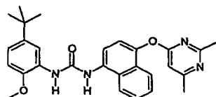
1-(5-tert-Butyl-2-methoxy-phenyl)-3-[4-(2,6-dimethyl-pyrimidin-4-yloxy)-naphthalen-1-yl]-urea;
